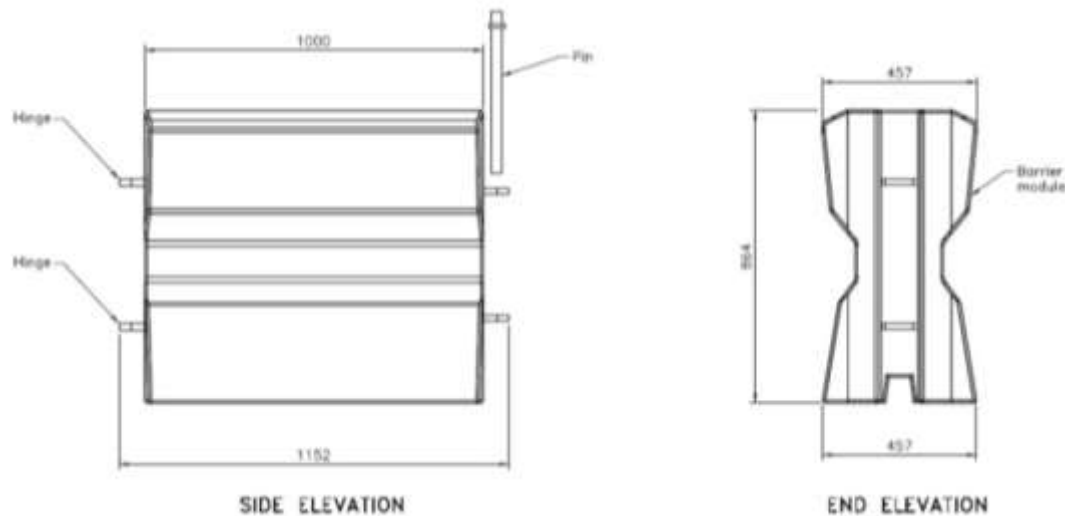
Figure 5-143: FLUX Barrier Dimensions
