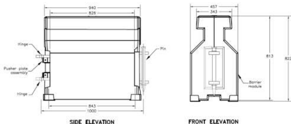
Figure 5-121: Reactive Tension System
