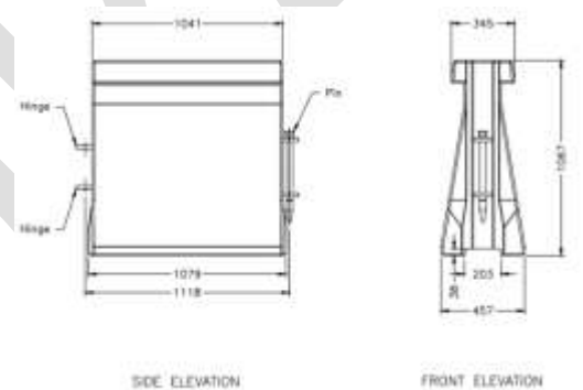
Figure 5-16XX: TALL42 Moveable Barrier Dimensions
