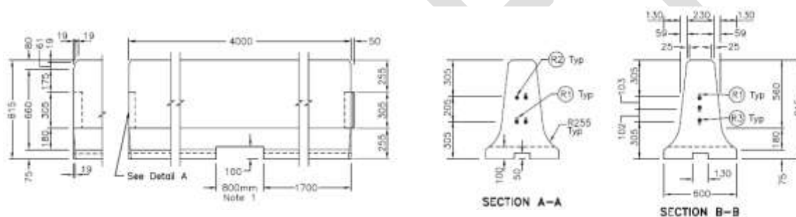
Figure 5-4: Type T Temporary Concrete Barrier
