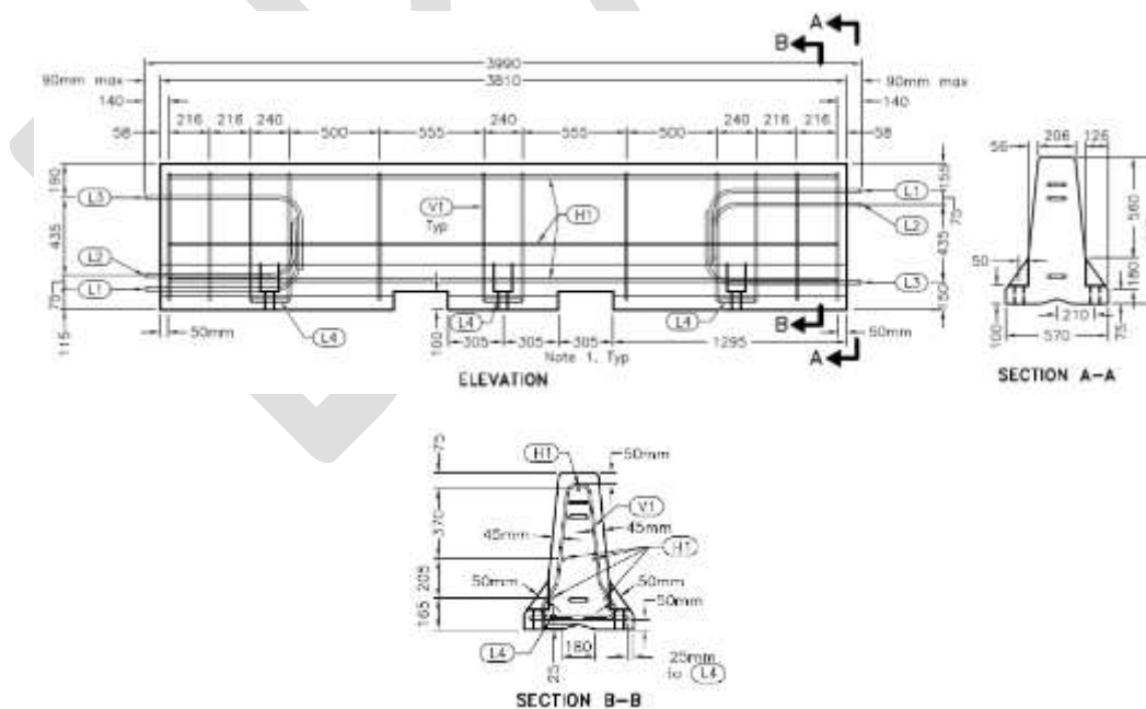
Figure 5-3: Type M Temporary Concrete Barrier
