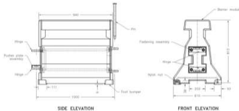
Figure 5-109: Quickchange Movable Barrier System
