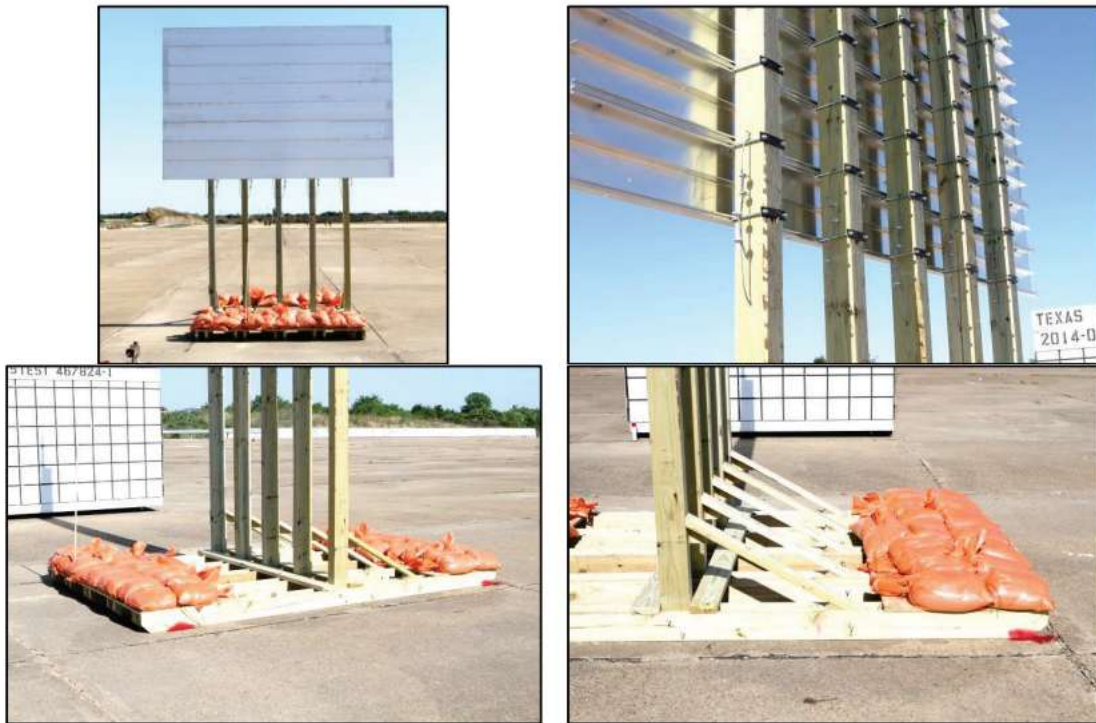
Figure 5-3128: Skid-Mounted Temporary Sign Support
