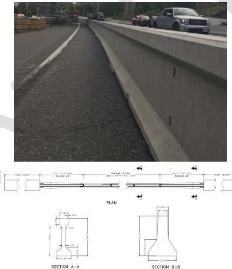
Figure 5-7: Type Z Temporary Concrete Barrier
