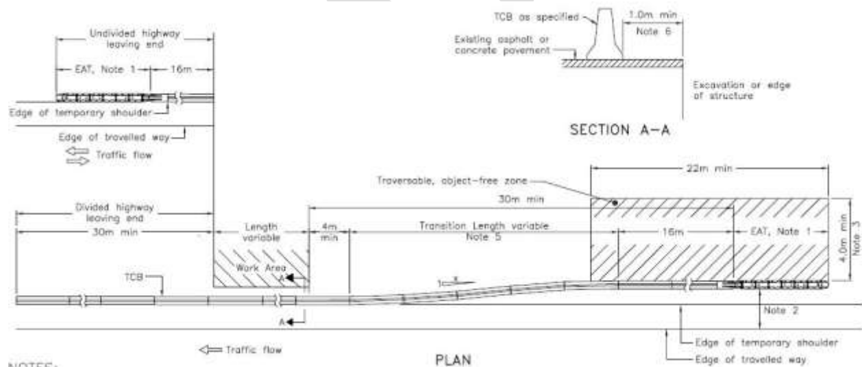
Figure 5-241: Typical TCB Layout with Temporary Reduced Exposure Energy Attenuator.
