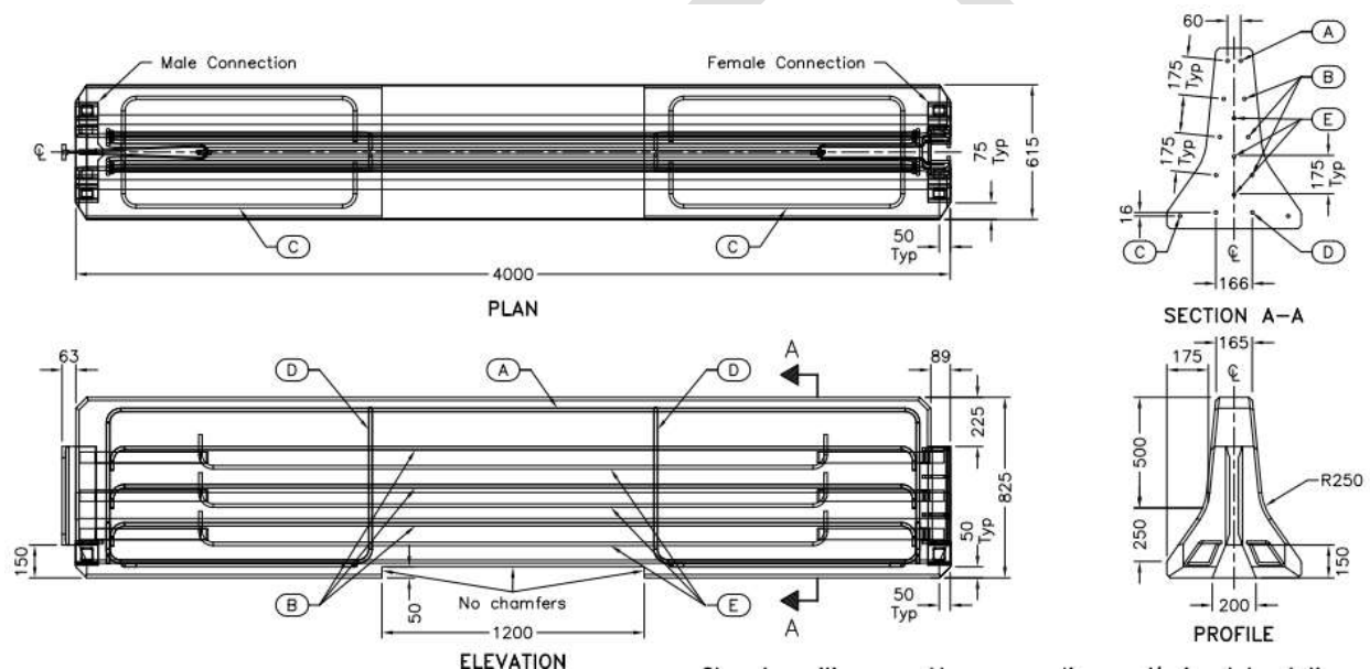
Figure 5-8X: Type H Temporary Concrete Barrier
