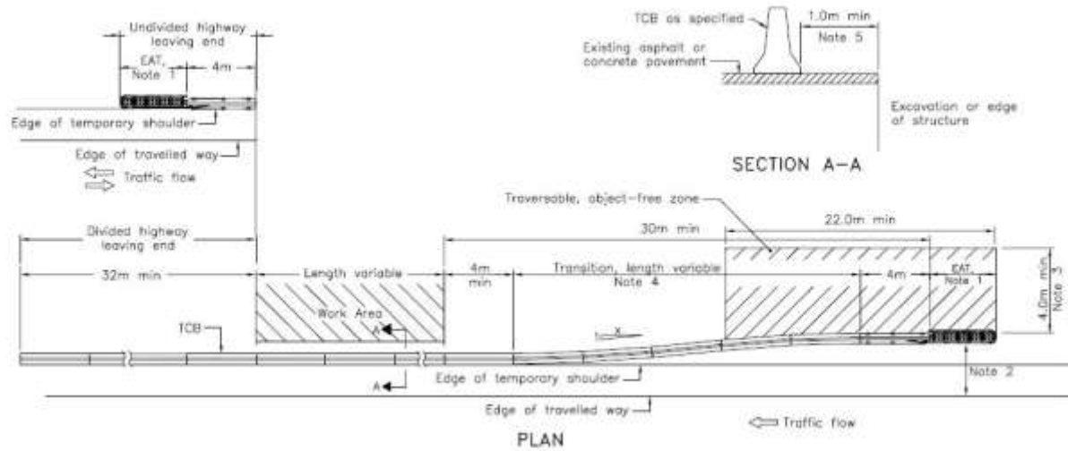
Figure 5-230: Typical TCB Layout with Temporary Energy Attenuator.
