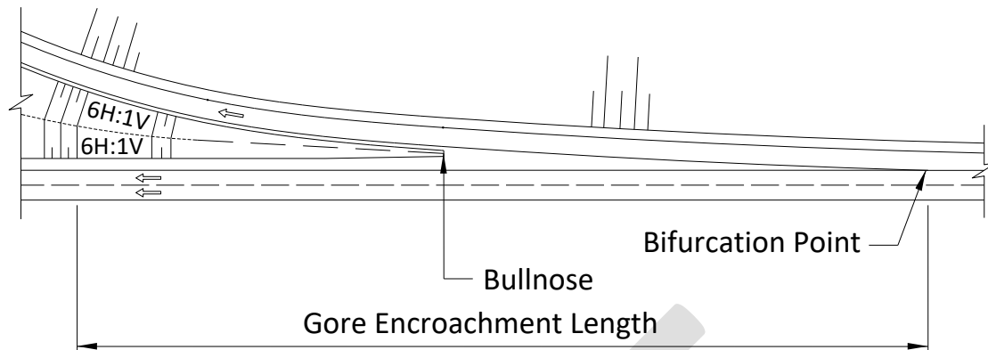
Figure 2-143: Clear Traversable Area Beyond Ramp Bullnose
