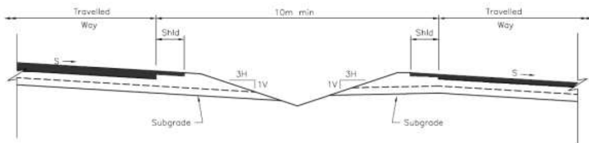
Figure 2-1: Desirable Grading Section for Medians Separating Low-Speed Interchange Ramps
