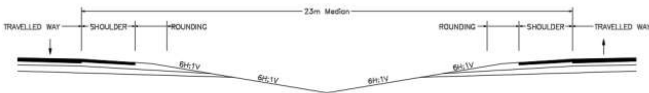
Figure 2-9: Minimum Median Configuration
