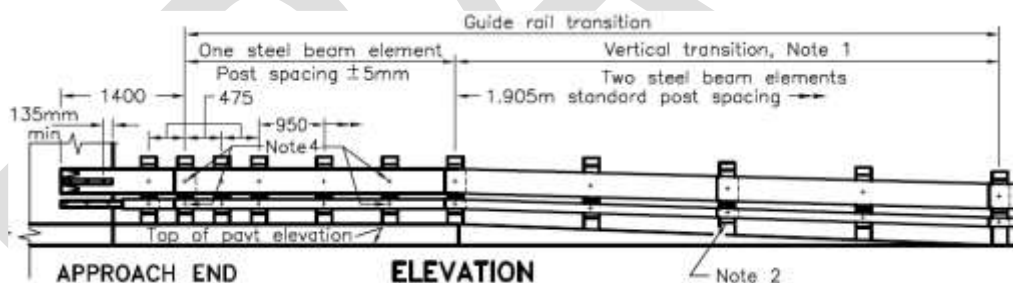
Figure 2-176: Legacy SBGR Connection to Rigid Barrier
