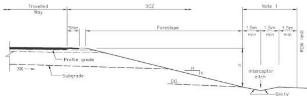
Figure 2-2: Earth/Shale Fill Sections To be used with Table 2-74
