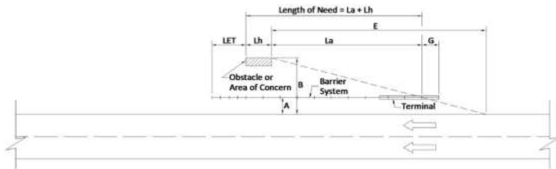
Figure 2-154: Length of Need – Divided Highway
