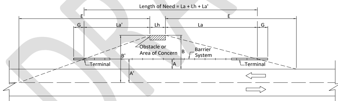
Figure 2-165: Length of Need – Undivided Highway
