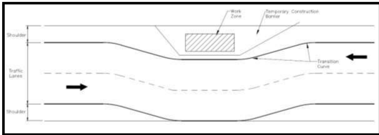
Exhibit- 13F Use of Shoulder with a Lane Shift
