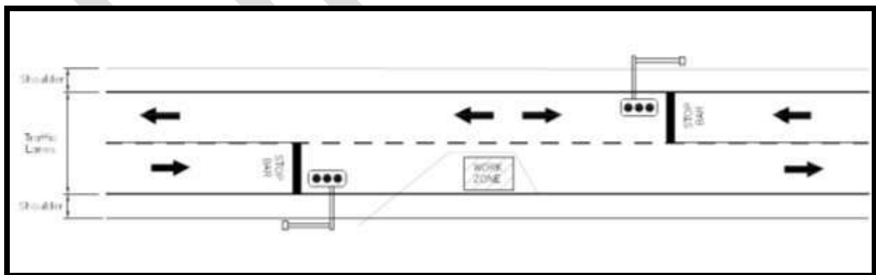
Exhibit- 13G Alternating One-way Operation Traffic flow on a Two-Lane Road Using Traffic Signal
