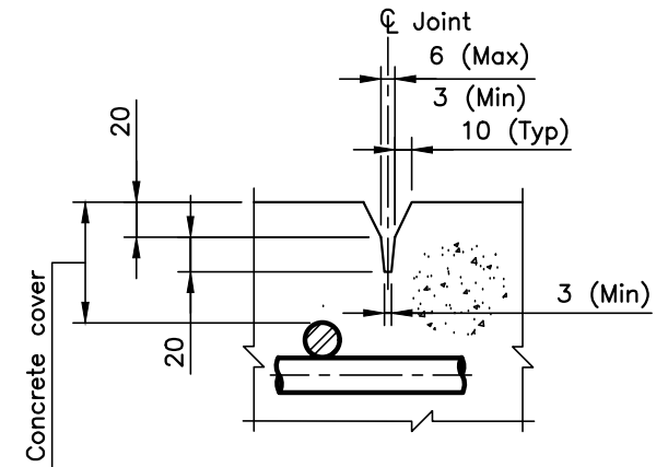
A CONTROL JOINT
