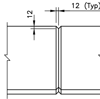
TYPICAL OPTIONAL CONSTRUCTION JOINT
