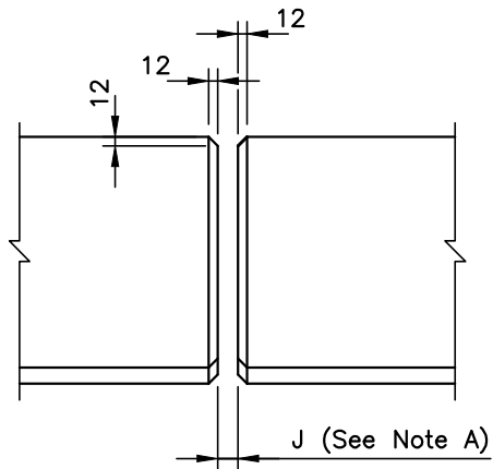
TYPICAL EXPANSION JOINT
