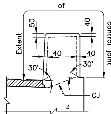
EXTENT OF CONTROL JOINT IN PARAPET WALL
