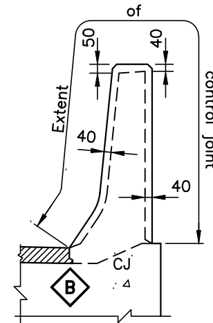
EXTENT OF CONTROL JOINT IN BARRIER WALL
