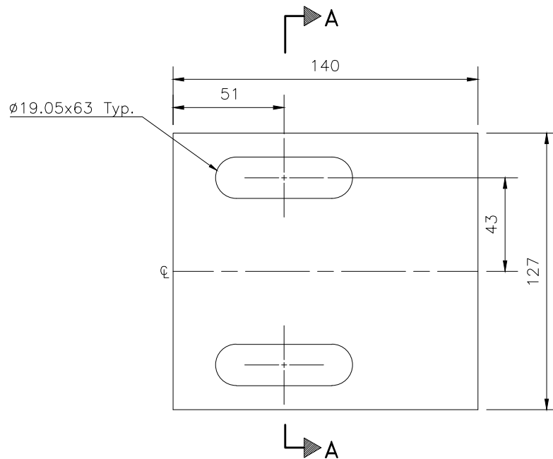
MOUNTING PLATE, Note 1
