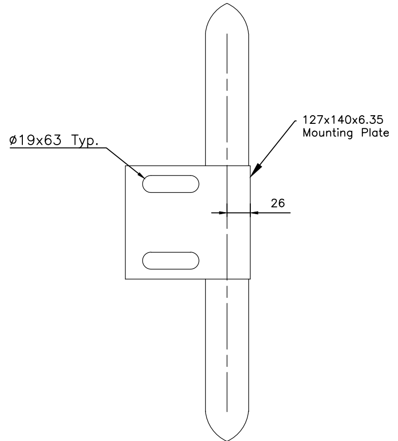
STEEL BLOCKOUT
