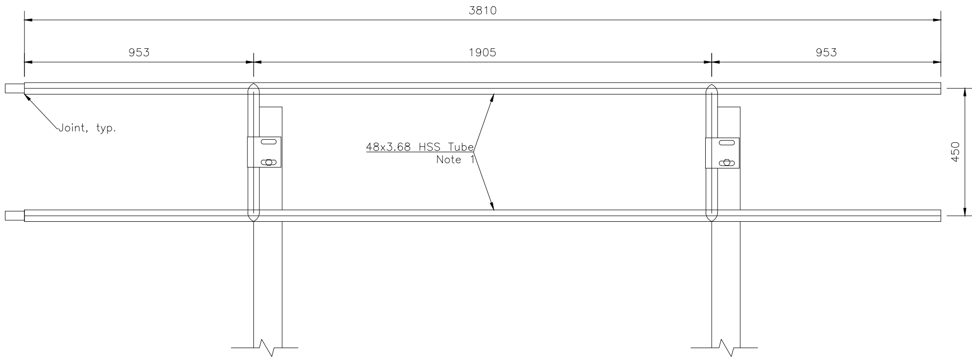
MIDSPAN ASSEMBLY
