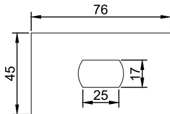
RECTANGULAR WASHER
