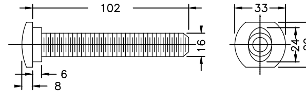
SPLICE BOLT
