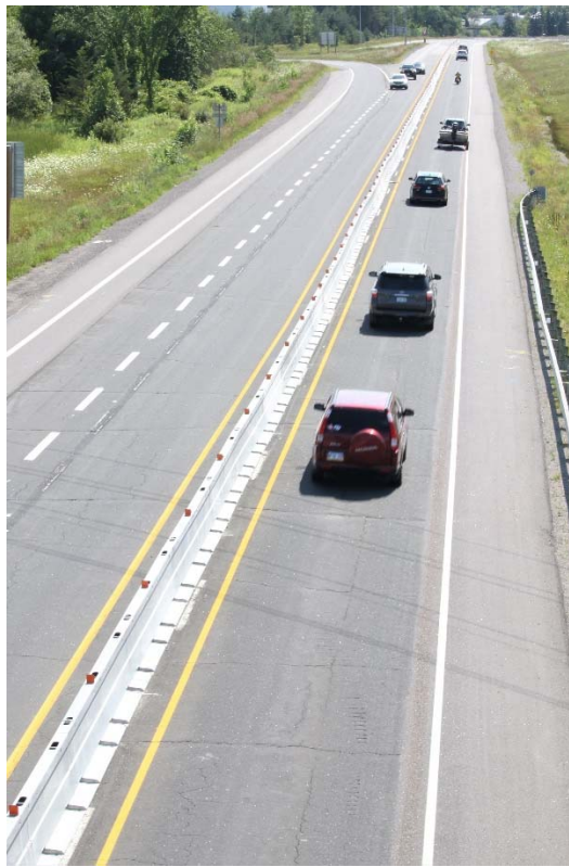
Figure 5-1: Category IV Barrier Separating Staged Opposing Freeway Traffic
