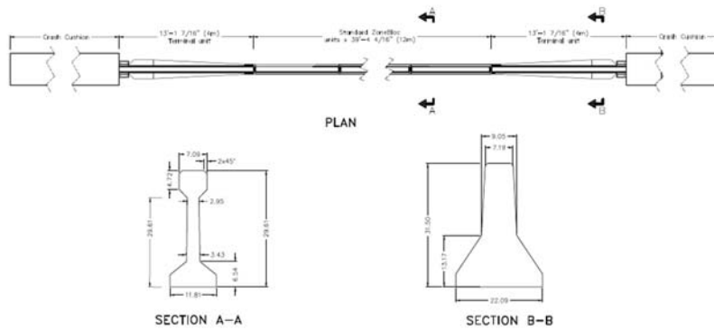
Figure 5-57: Type Z Temporary Concrete Barrier
