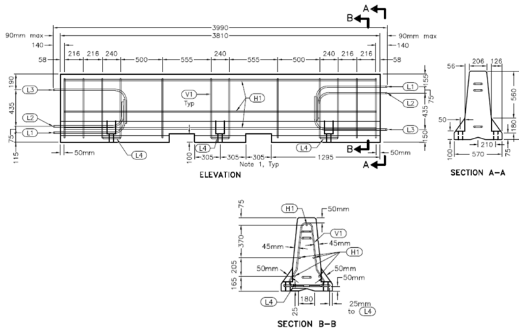
Figure 5-23: Type M Temporary Concrete Barrier
