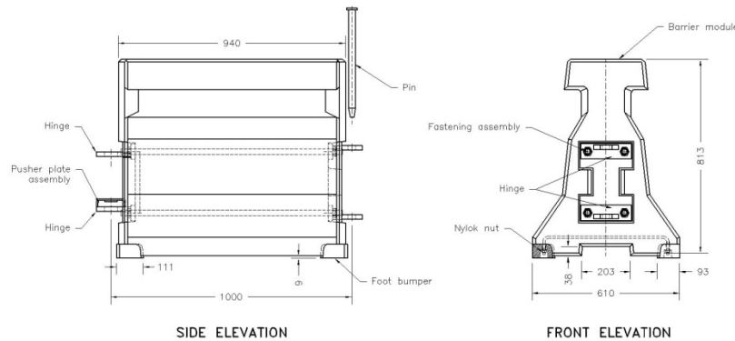
Figure 5-97: Quickchange Movable Barrier System
