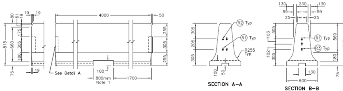
5-34: Type T Temporary Concrete Barrier
