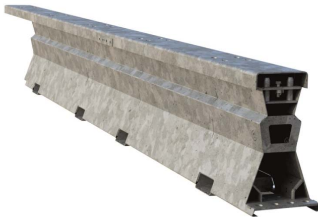
Figure 5-171: Safezone Barrier Photo courtesy of Laura Metaal
