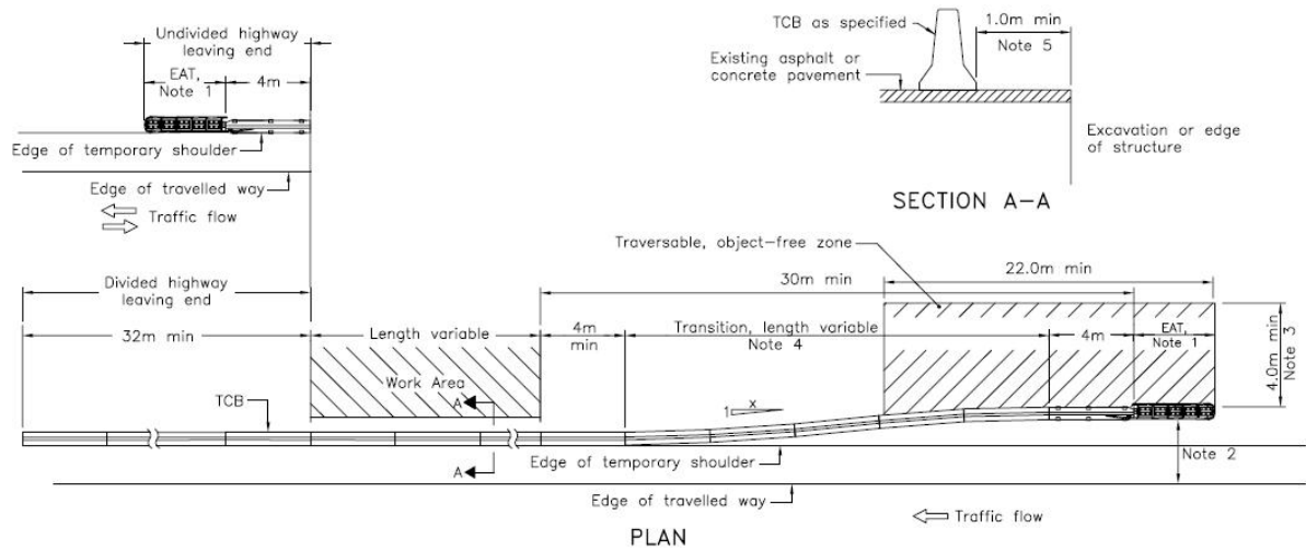
Figure 5-1320: Typical TCB Layout with Temporary Energy Attenuator. See applicable standard for Notes
