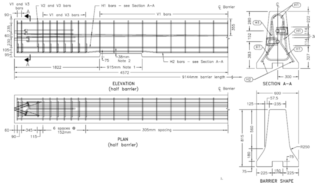
Figure 5-45: Type X Temporary Concrete Barrier
