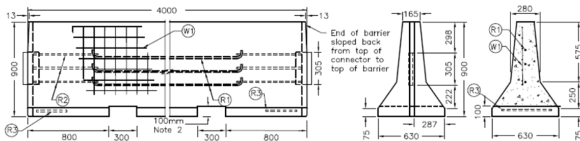
Figure 5-12: Type J Temporary Concrete Barrier
