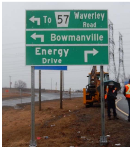
Figure 4-4047: SlipSafe Supreme Intermediate Sign Support System Installation
