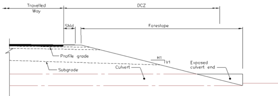
Figure 4-4451: Exposed Culvert End within Desirable Clear Zone
