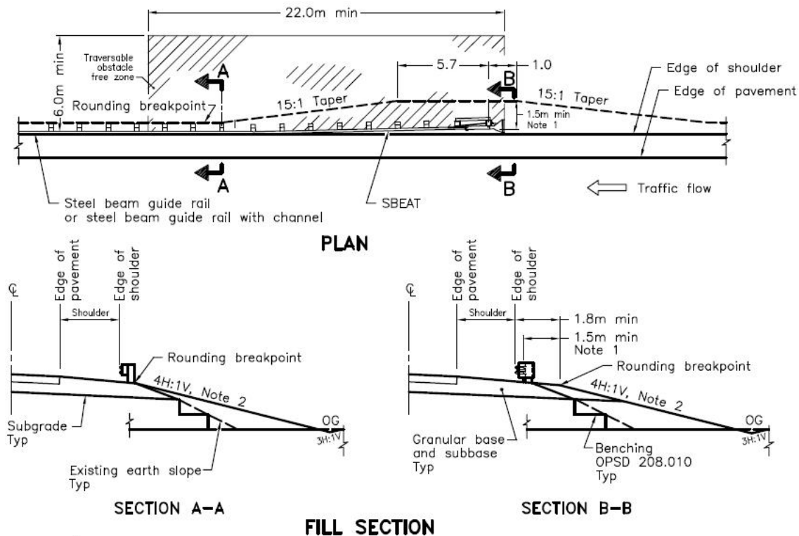
Figure 4-2125: Desirable Grading for SBEAT Installations
