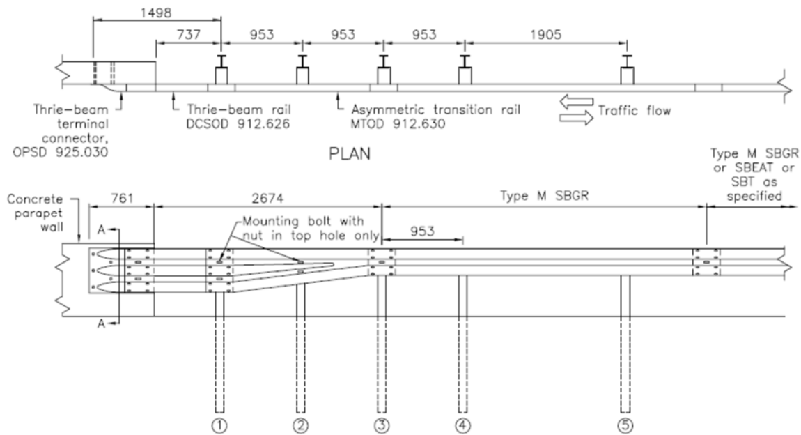
Figure 4-1112: Type M MASH TL-2 SBGR Connection to Rigid Barrier on Low Speed Roads
