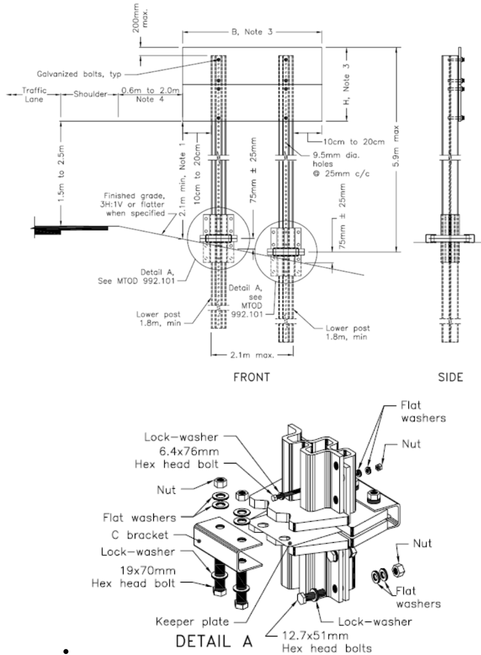
Figure 4-4148: Breakaway Component Details
