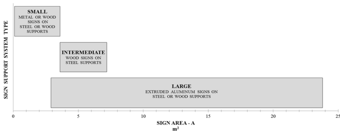
Figure 4- 36 43 : Sign Support System Types and Sign Areas
