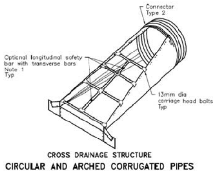
Figure 4-4552: Culvert End with Safety Slope End Treatment
