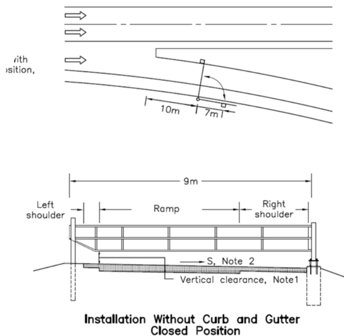
Figure 4-43-50: Breakaway Ramp Closure gate installed on ramp without curb. Gate shown in ramp closed position.
