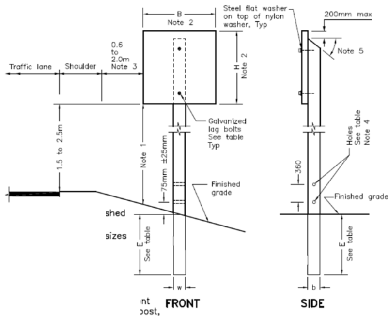
Figure 4-3744: Small Breakaway Single Post System with 89 mm x 140 mm Drilled Wooden Post.
