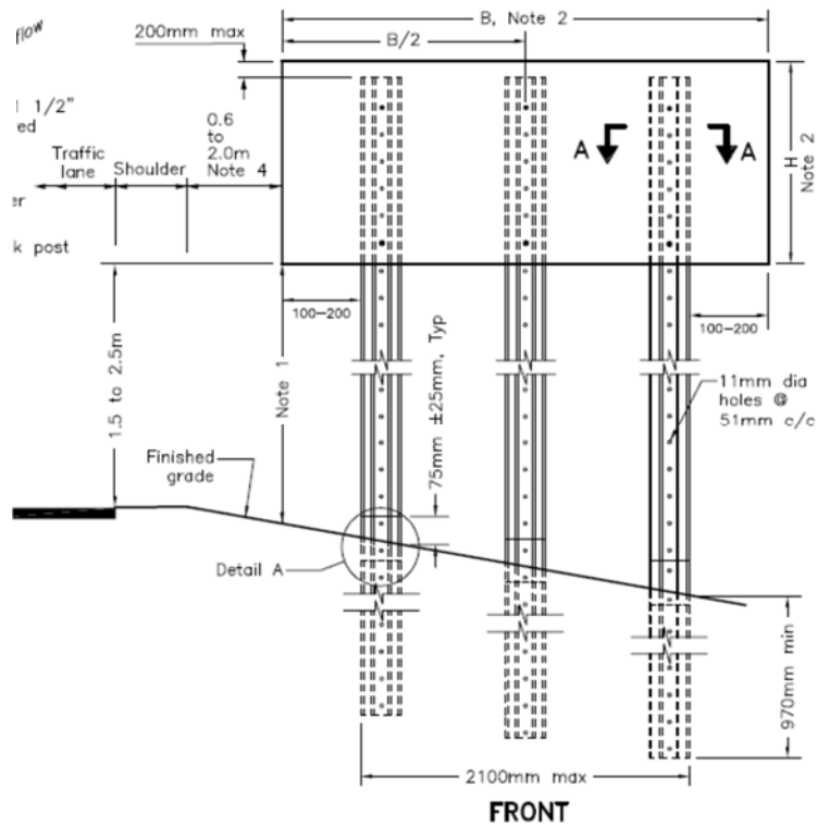
Figure 4-3845: Small Breakaway Triple Post System with Rib-Bak steel posts See applicable standards for other post configurations and note references.
