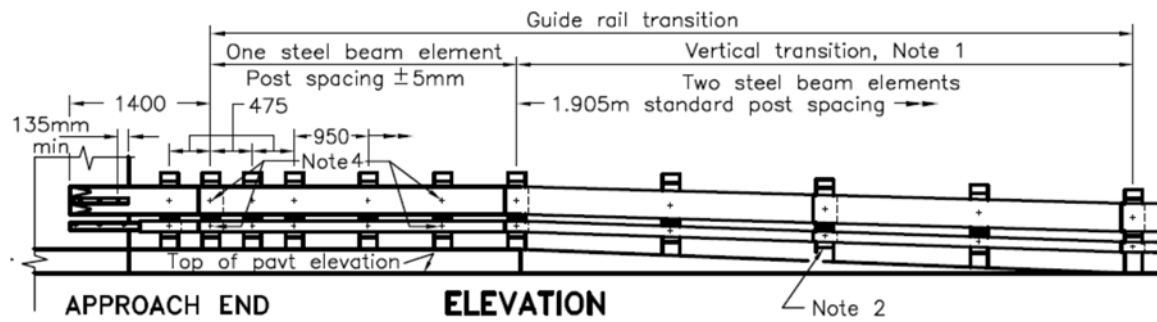
Figure 4-1011: Standard SBGR Connection to Rigid Barrier
