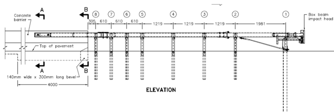
Figure 4-3136: Box Beam Bursting Energy Absorbing Terminal
