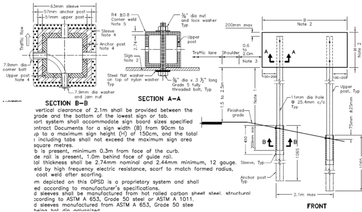
Figure 4-3946: Small Breakaway Double Post System with Sqr-Loc steel posts See applicable standards for other post configurations and note references.
