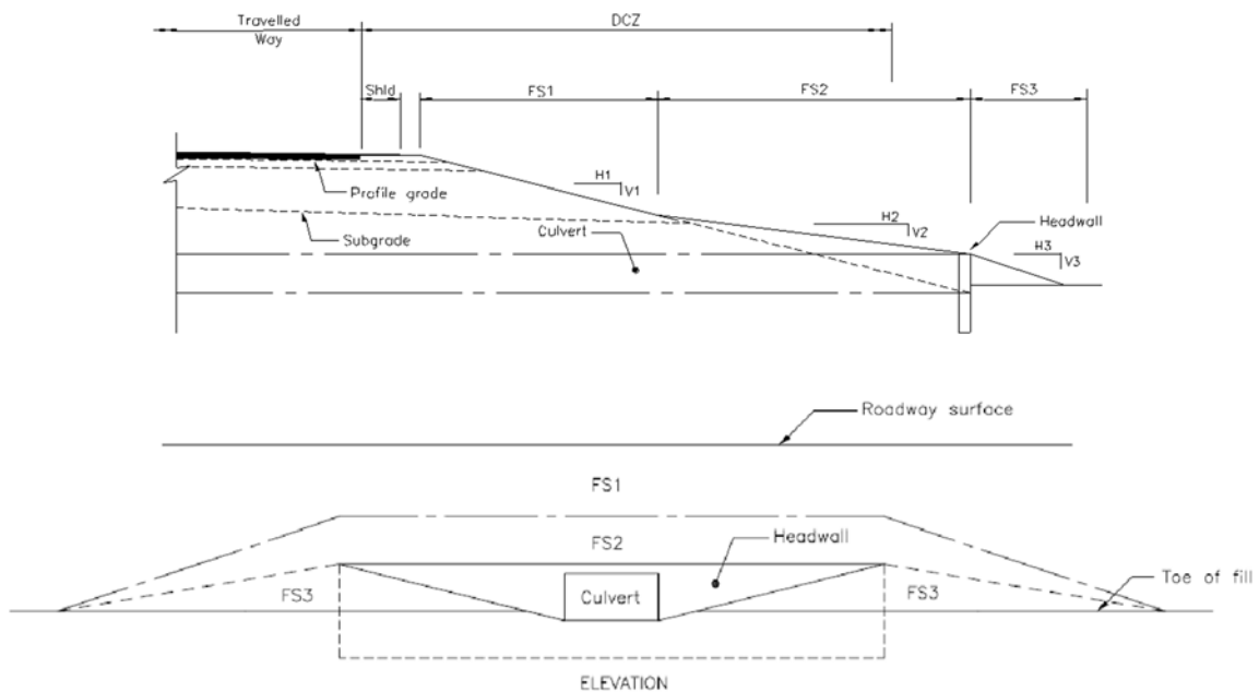
Figure 4-4653: Culvert End with Headwall
