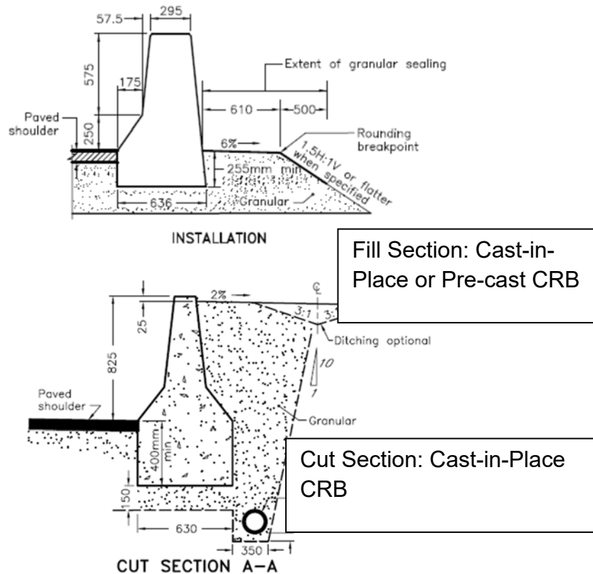
Figure 4-1415: Concrete Roadside Barrier Installations
