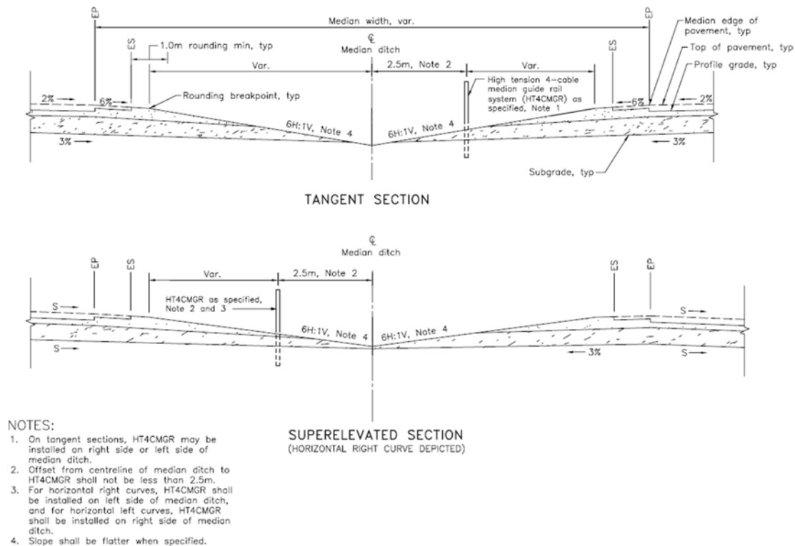
Figure 4-1620: Typical HT4CMGR installation for rural median with 6H:1V slopes
