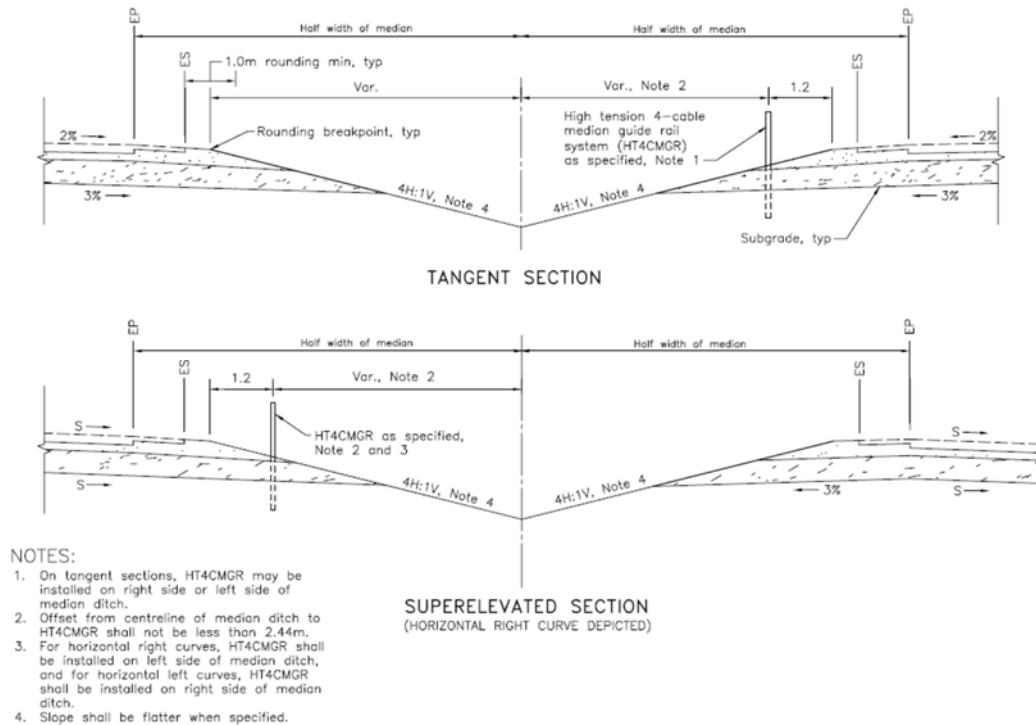
Figure 4-1519: Typical HT4CMGR installation for rural median with 4H:1V slopes
