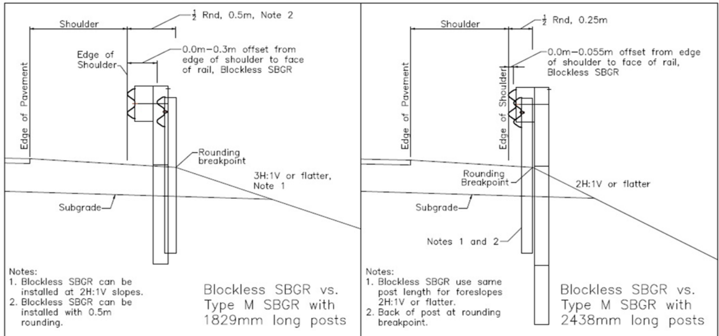
Figure 4-1314: Blockless SBGR Compared to M20 SBGR at Rounding Breakpoint
