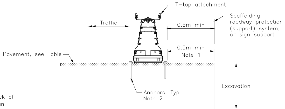
END VIEW
