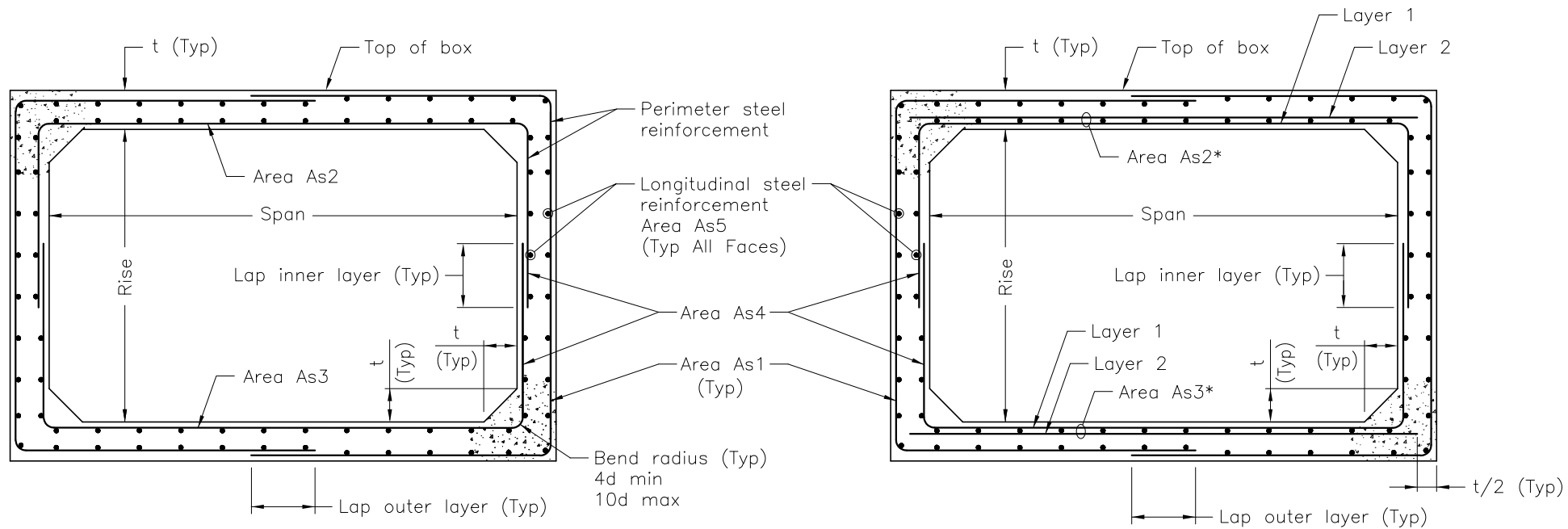
LAYOUT 1: SINGLE LAYER OF REINFORCEMENT
